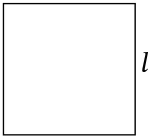
Square
