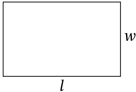
Rectangle
