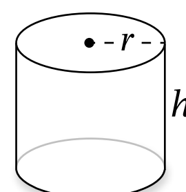
Cylinder
