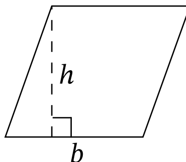
Parallelogram
