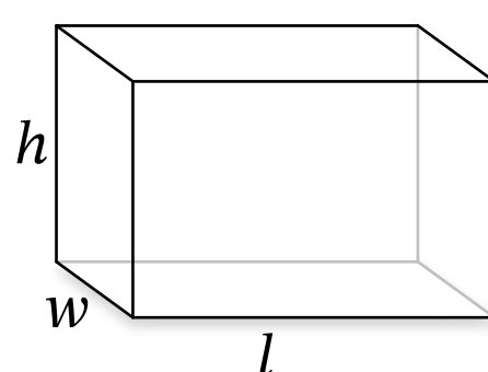
Rectangular Prism
