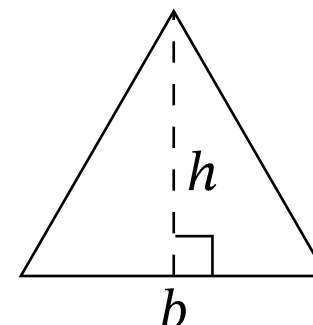
Triangle
