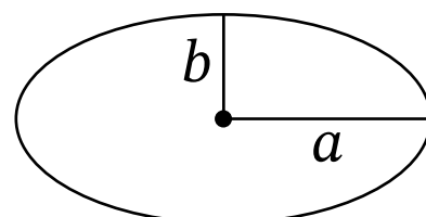
Ellipse
