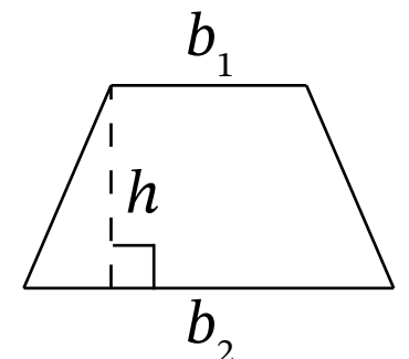
Trapezoid
