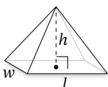
Rectangular Pyramid
